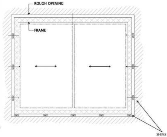
Horizontal Slider
