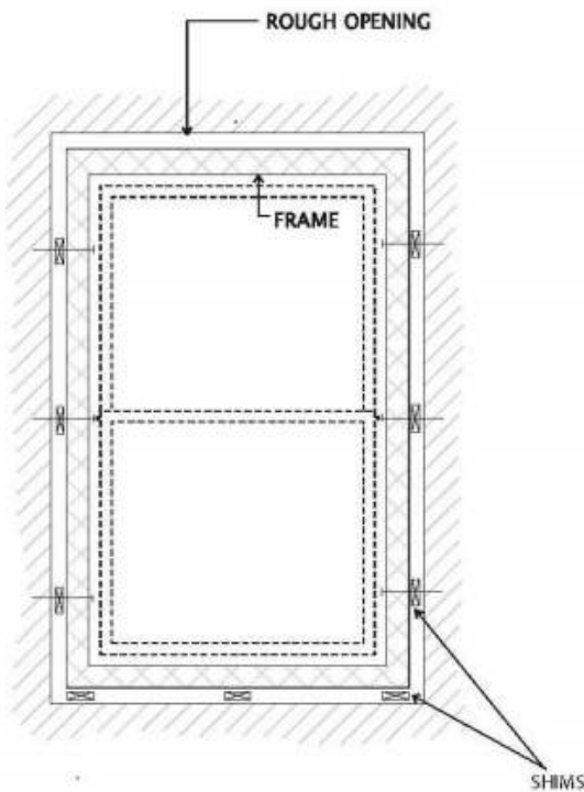
Vertical Slider
