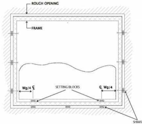
Fixed Windows
