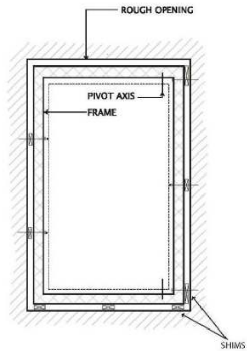
Casement
